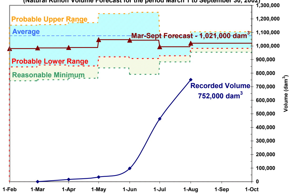
Water Supply Forecast as of August 1, 2002 for the Bow River at Banff (Natural Runoff Volume Forecast for the period March 1 to September 30, 2002)
