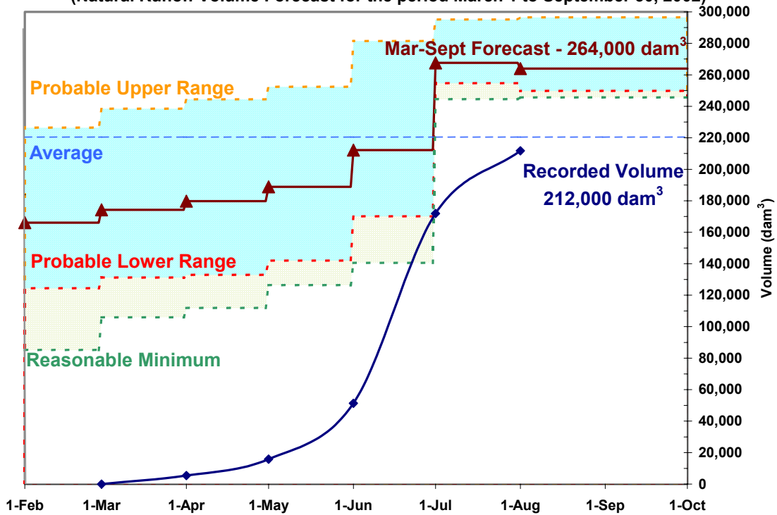
Water Supply Forecast as of August 1, 2002 for the Elbow River at Bragg Creek (Natural Runoff Volume Forecast for the period March 1 to September 30, 2002)
