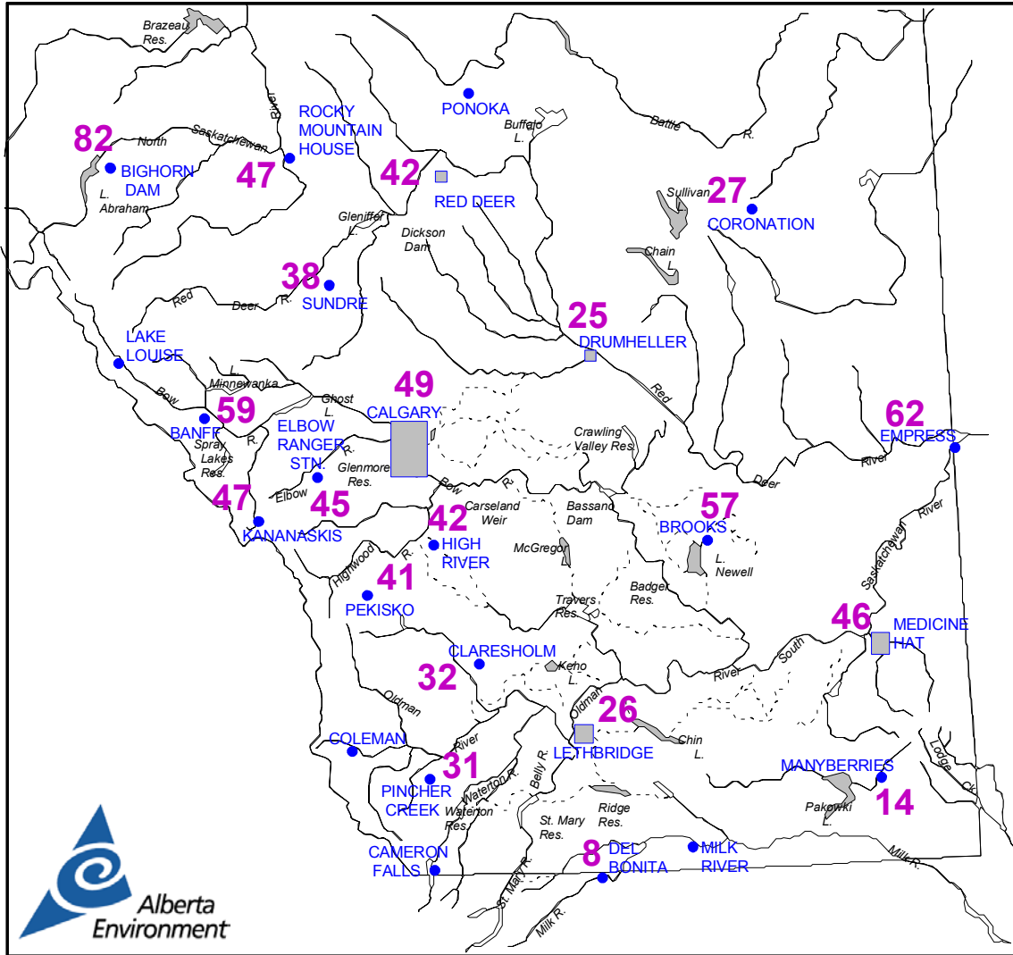
Figure 11 Precipitation Southern Alberta September 1, 2001 to October 31, 2001 as a percent of Normal Normal = 100% (based on 1961 to 1990 data)
