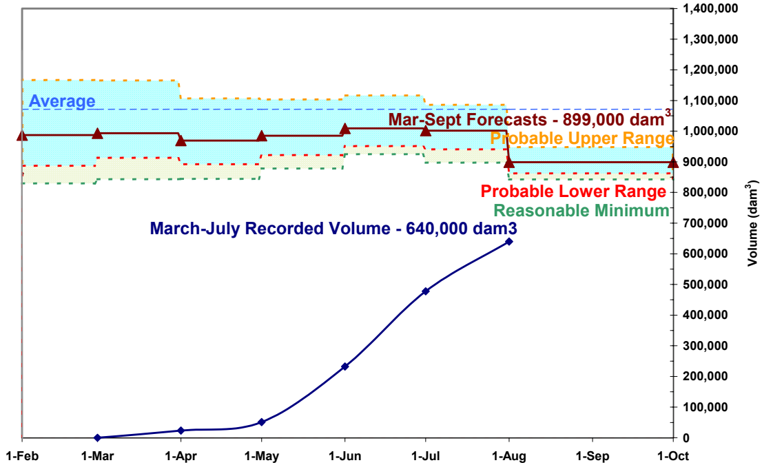
Water Supply Forecast as of August 1, 2006 for the Bow River at Banff (Natural Runoff Volume Forecast for the period March 1 to September 30, 2006)
