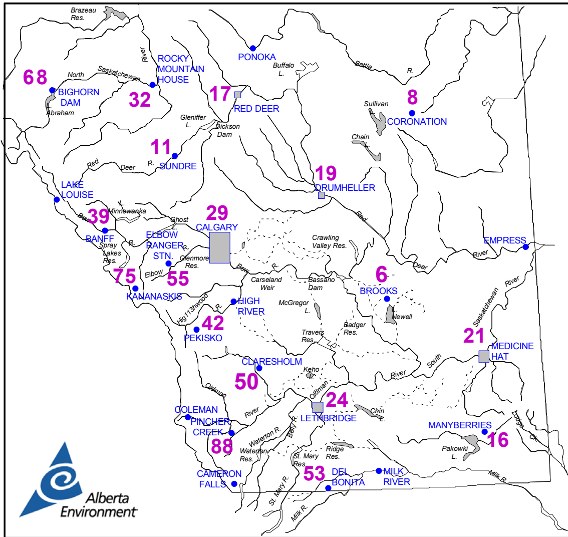
Figure 2 Precipitation Southern Alberta November 1 to 30, 2004 as a percent of Normal Normal = 100% (based on 1961 to 1990 data)
