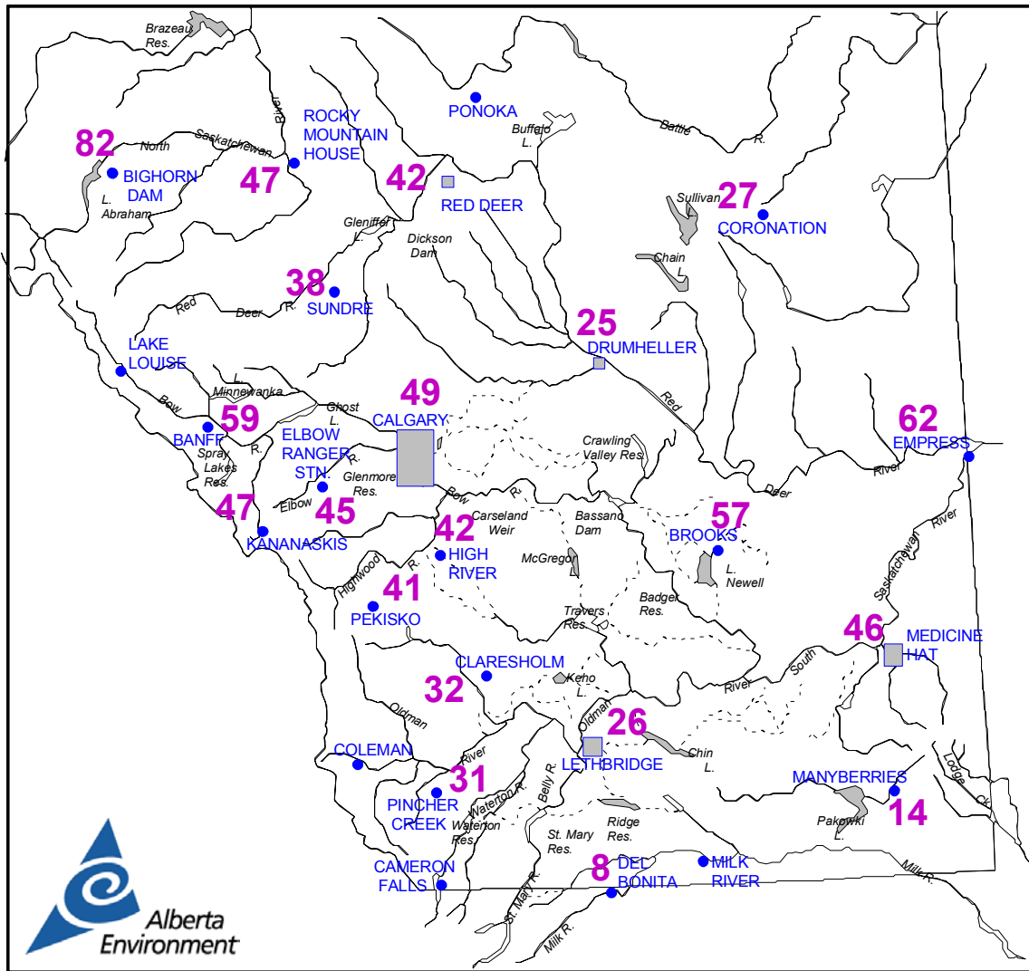
Figure 2 Precipitation Southern Alberta September 1, 2001 to October 31, 2001 as a percent of Normal Normal = 100% (based on 1961 to 1990 data)
