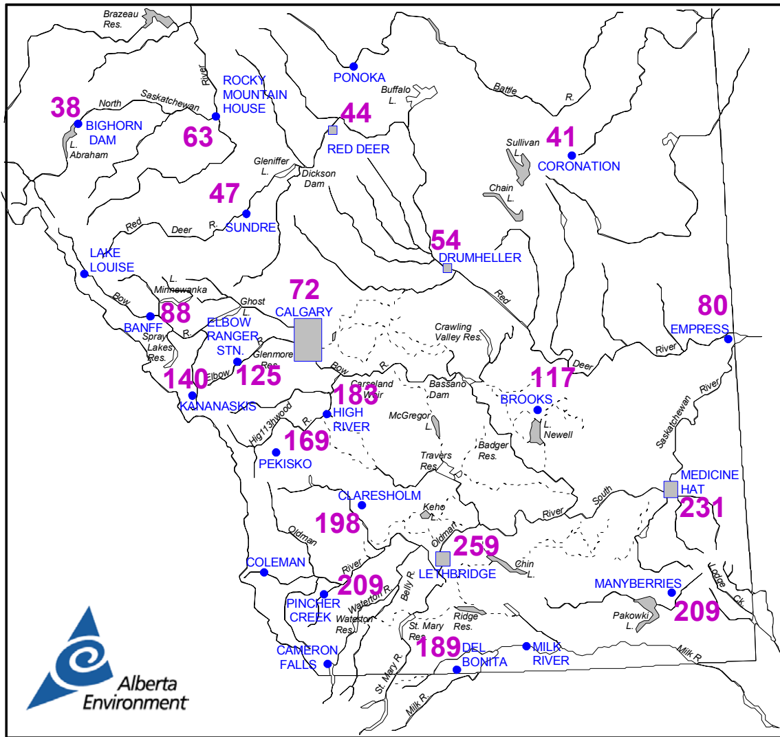
Figure 5 Precipitation Southern Alberta May 1, 2002 to June 30, 2002 as a percent of Normal Normal = 100% (based on 1961 to 1990 data)
