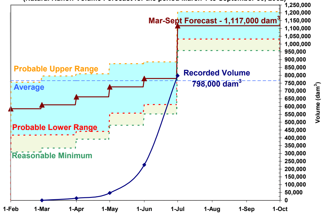
Water Supply Forecast as of July 1, 2002 for the St. Mary River at St. Mary Reservoir (Natural Runoff Volume Forecast for the period March 1 to September 30, 2002)
