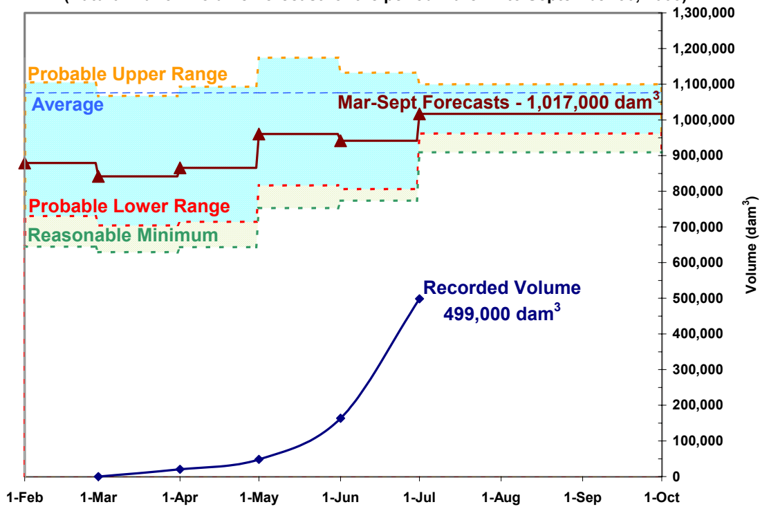
Water Supply Forecast as of July 1, 2003 for the Bow River at Banff (Natural Runoff Volume Forecast for the period March 1 to September 30, 2003)
