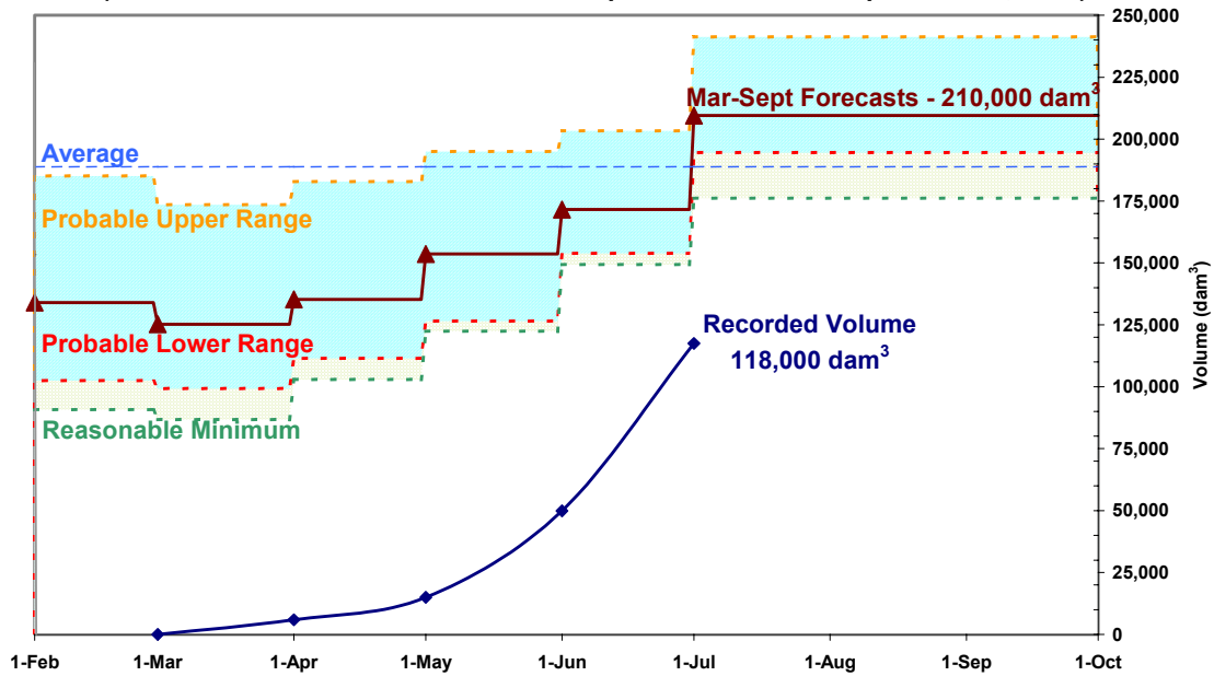
Water Supply Forecast as of July 1, 2003 for Lake Minnewanka Inflow (Natural Runoff Volume Forecast for the period March 1 to September 30, 2003)
