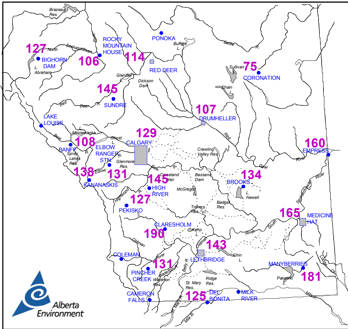
Figure 11 Precipitation Southern Alberta September 1, 2002 to October 31, 2002 as a percent of Normal Normal = 100% (based on 1961 to 1990 data)
