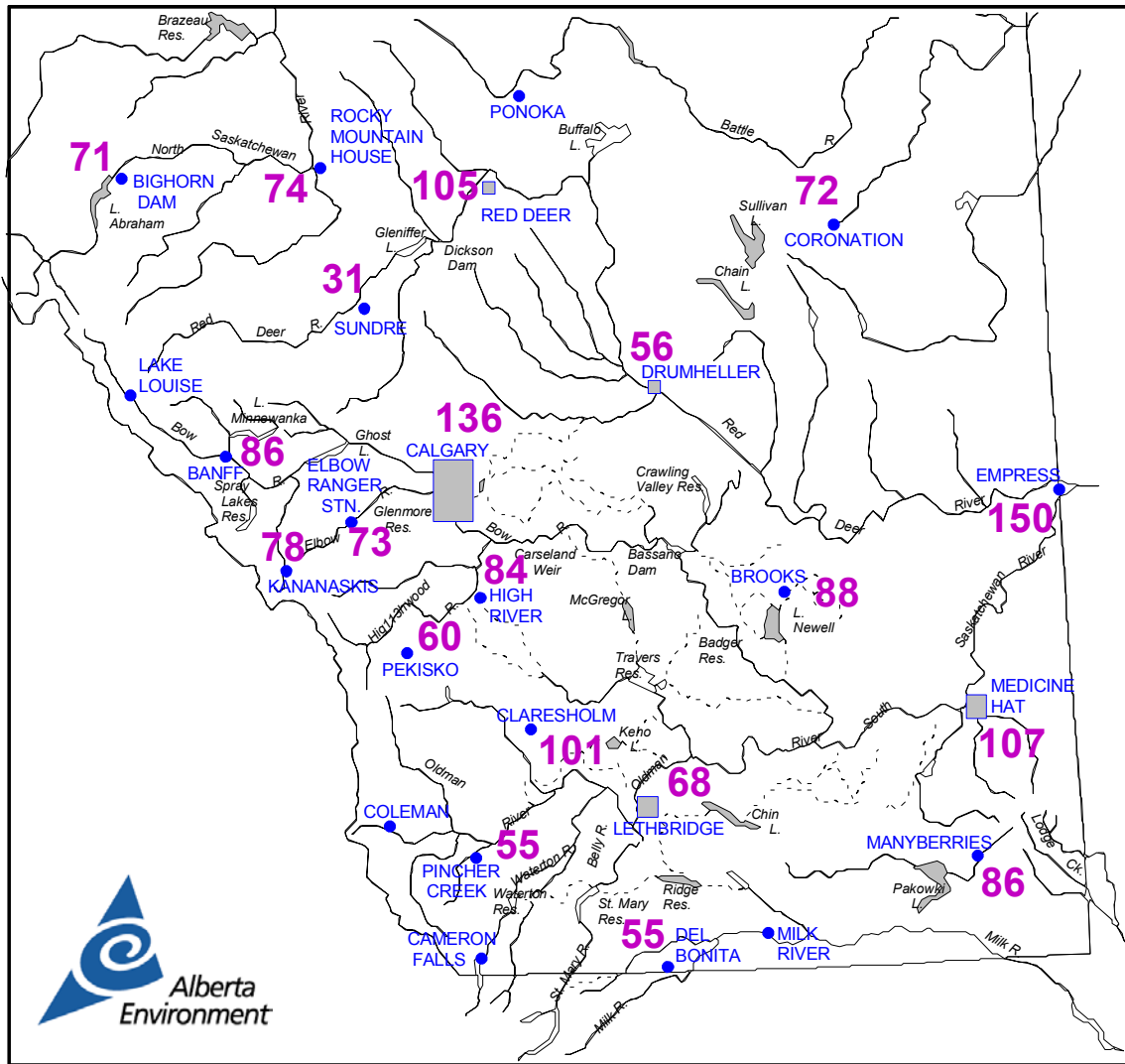
Figure 2 Precipitation Southern Alberta June 1 to 30, 2003 as a percent of Normal Normal = 100% (based on 1961 to 1990 data)
