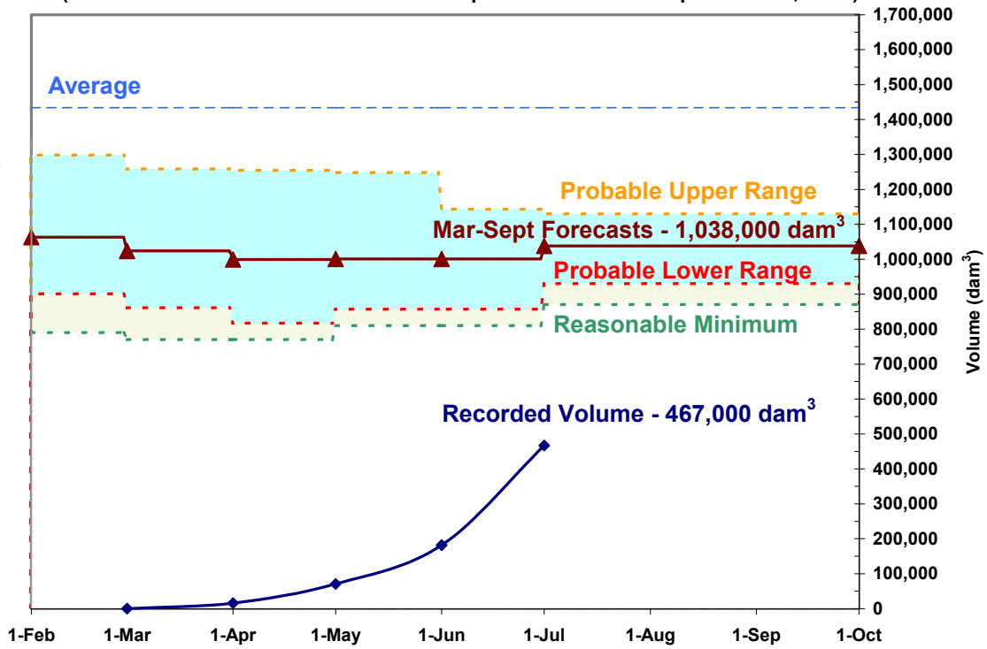
Water Supply Forecast as of July 1, 2004 for the Brazeau River at Brazeau Dam (Natural Runoff Volume Forecast for the period March 1 to September 30, 2004)
