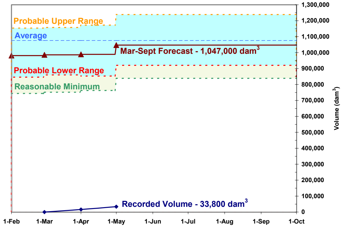
Water Supply Forecast as of May 1, 2002 for the Bow River at Banff (Natural Runoff Volume Forecast for the period March 1 to September 30, 2002)
