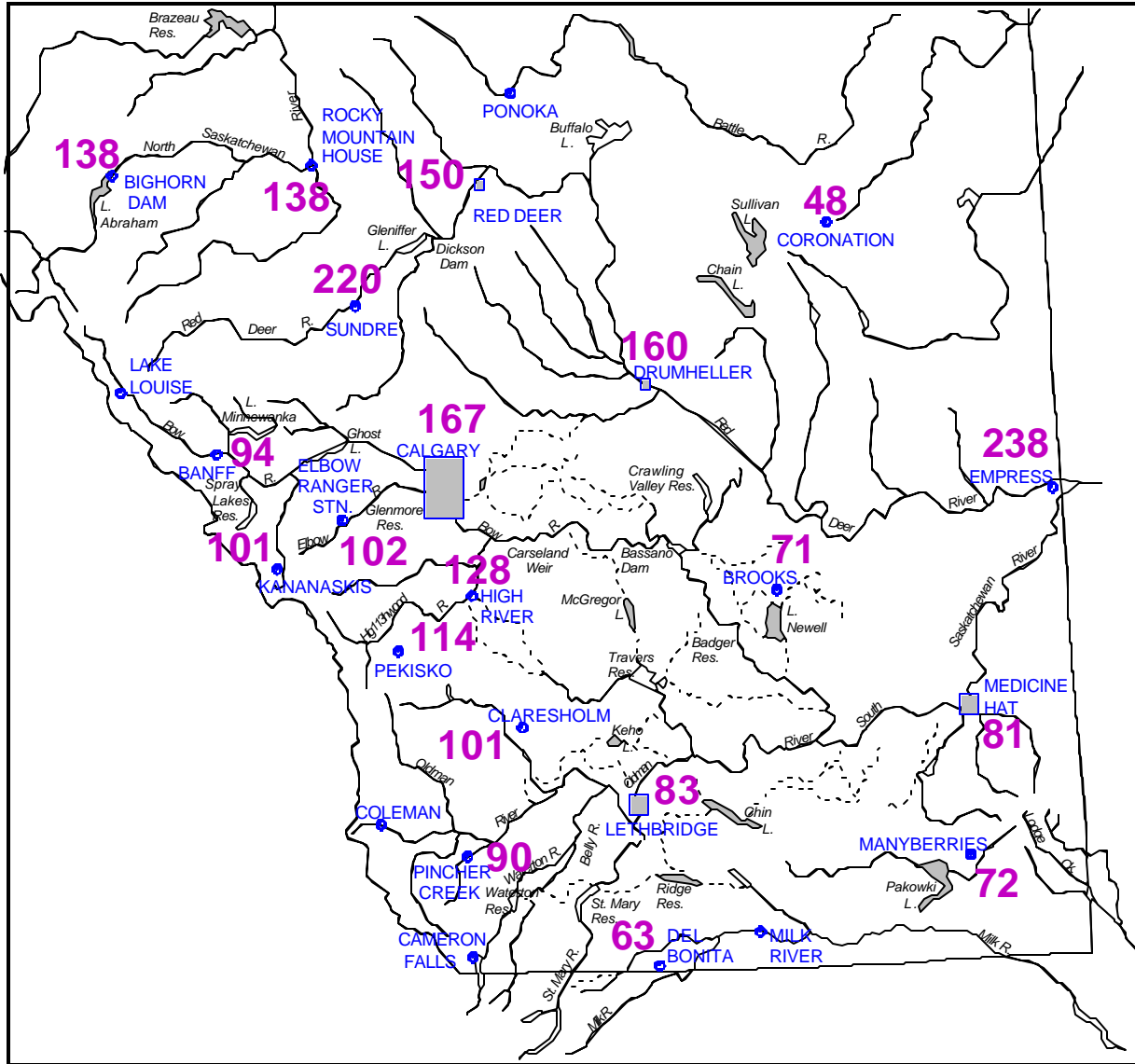
Figure 5 Precipitation Southern Alberta November 1, 2002 to April 30, 2003 as a percent of Normal Normal = 100% (based on 1961 to 1990 data)
