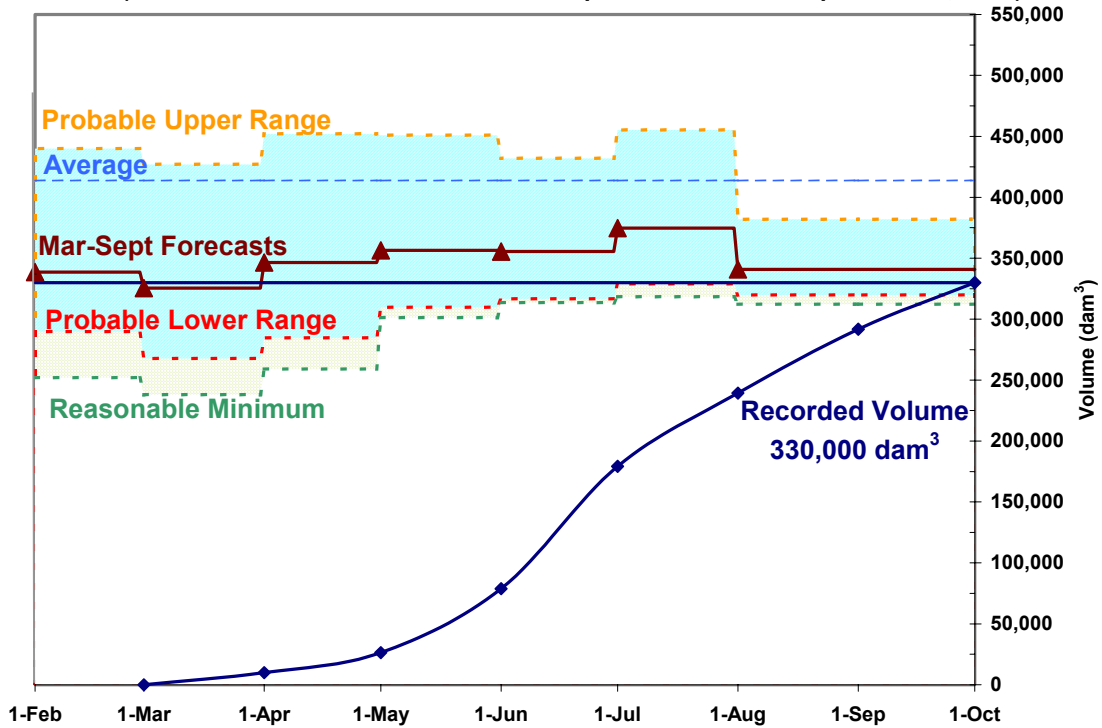
Water Supply Forecast as of October 1, 2003 for the Kananaskis River (Natural Runoff Volume Forecast for the period March 1 to September 30, 2003)
