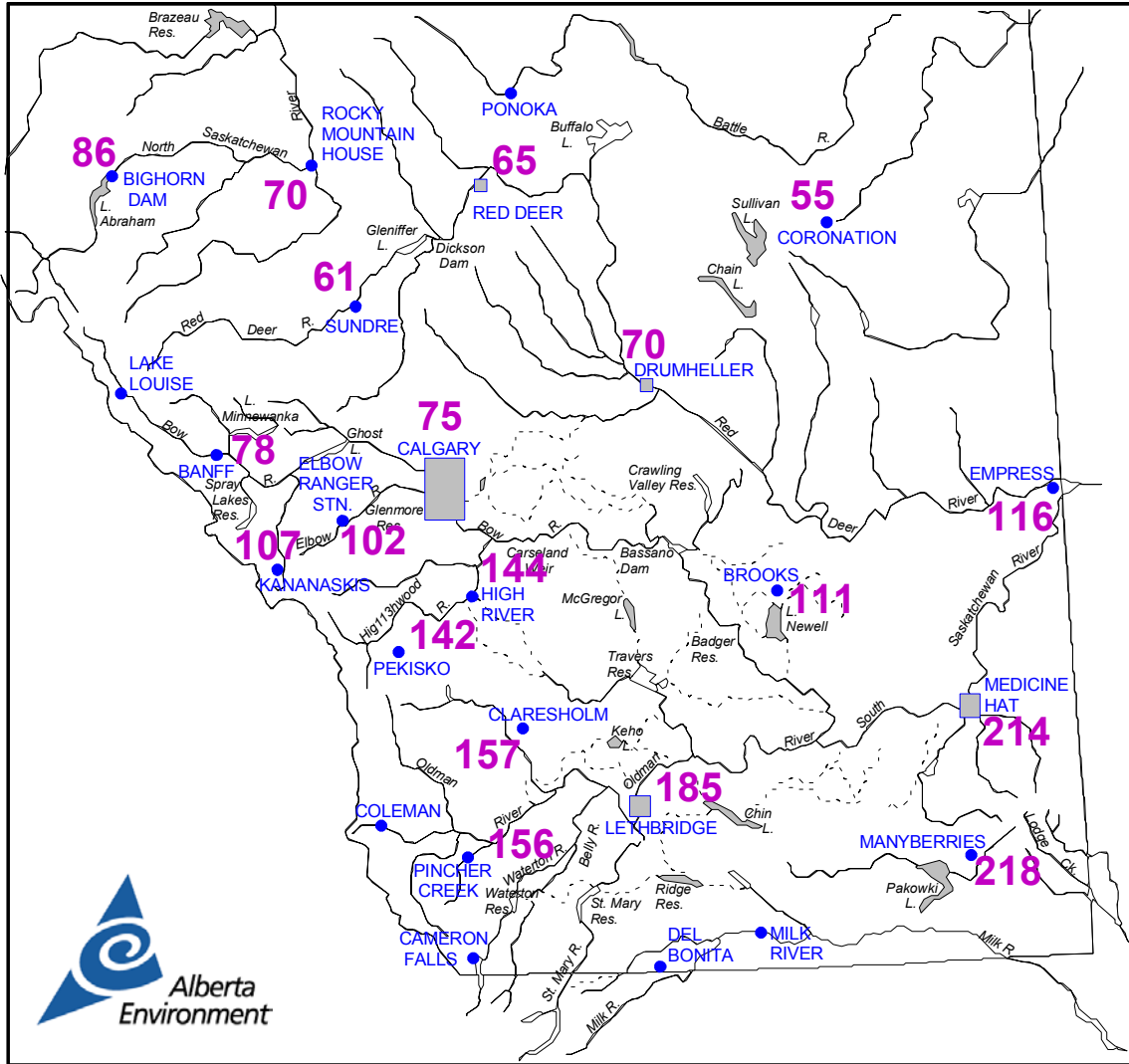
Figure 5 Precipitation Southern Alberta May 1, 2002 to August 31, 2002 as a percent of Normal Normal = 100% (based on 1961 to 1990 data)
